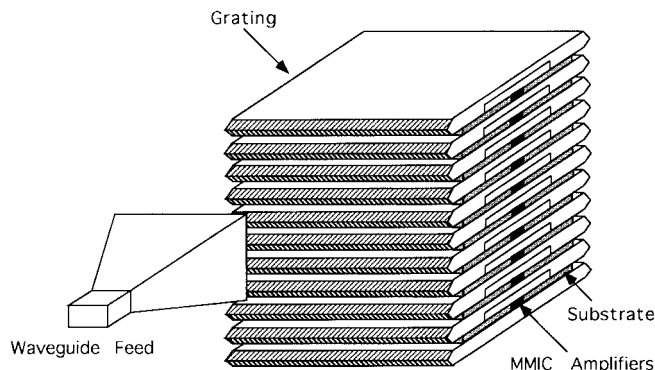
Fig. 1. Millimeter-wave quasi-optical MMIC amplifier array. The amplifiers are approximately spaced \lambda/2 apart in both the horizontal and vertical dimension at the operating frequency. Lenses (not shown) are used to focus the beam from the waveguide feed to the grating.
