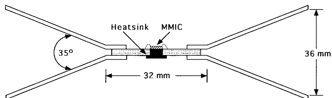
Fig. 2. Cross section of the 1 \times n amplifier array. The dielectric material stacked between the parallel plates has an \epsilon_r of 3.27 and a thickness of 0.381 mm. The MMIC's are bonded to the substrate using an ultrasonic bonder.
